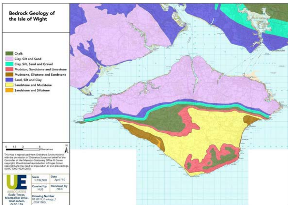
Figure 6.7: Geology of the Isle of Wight
