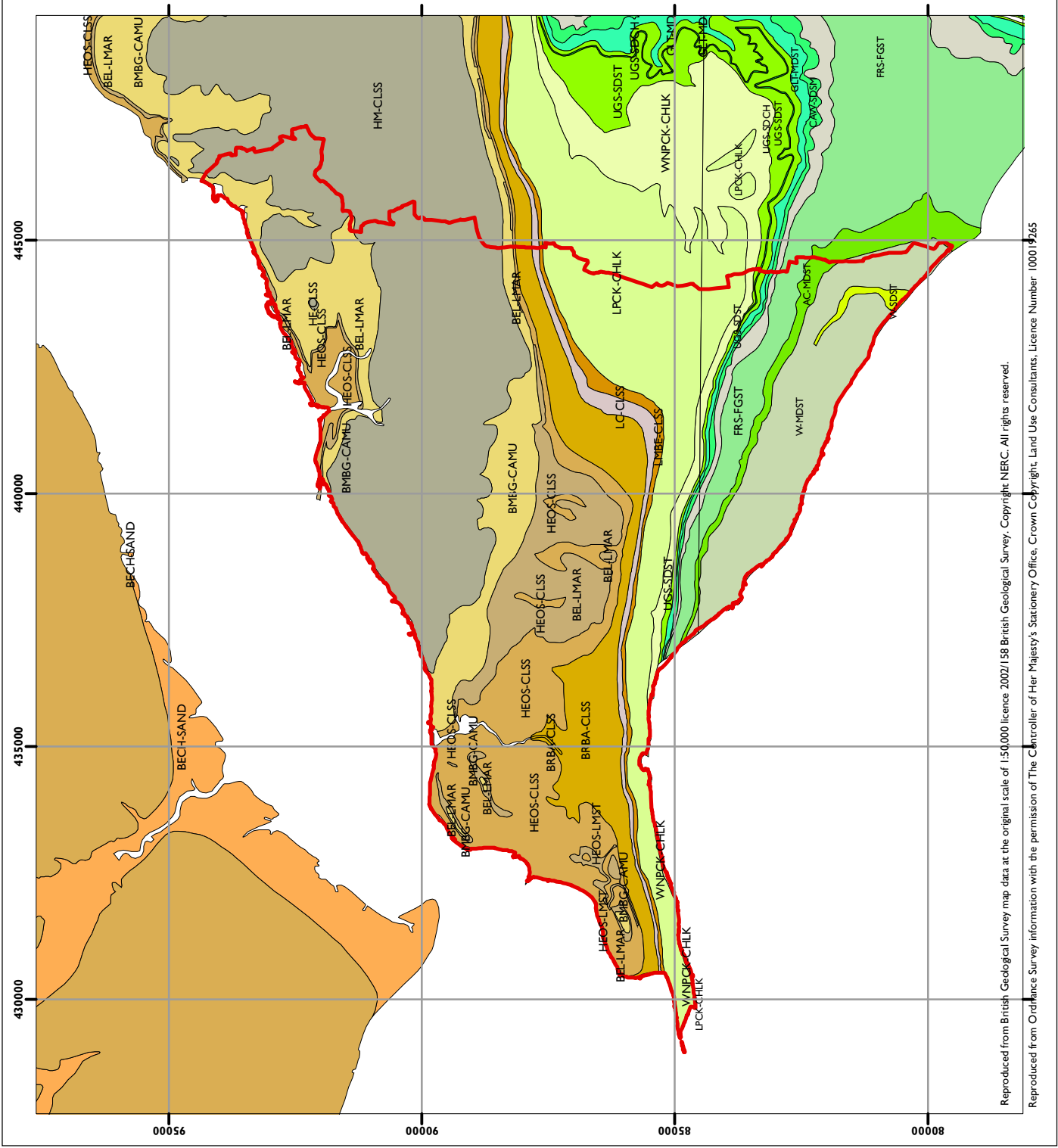
Figure 5: Solid Geology
