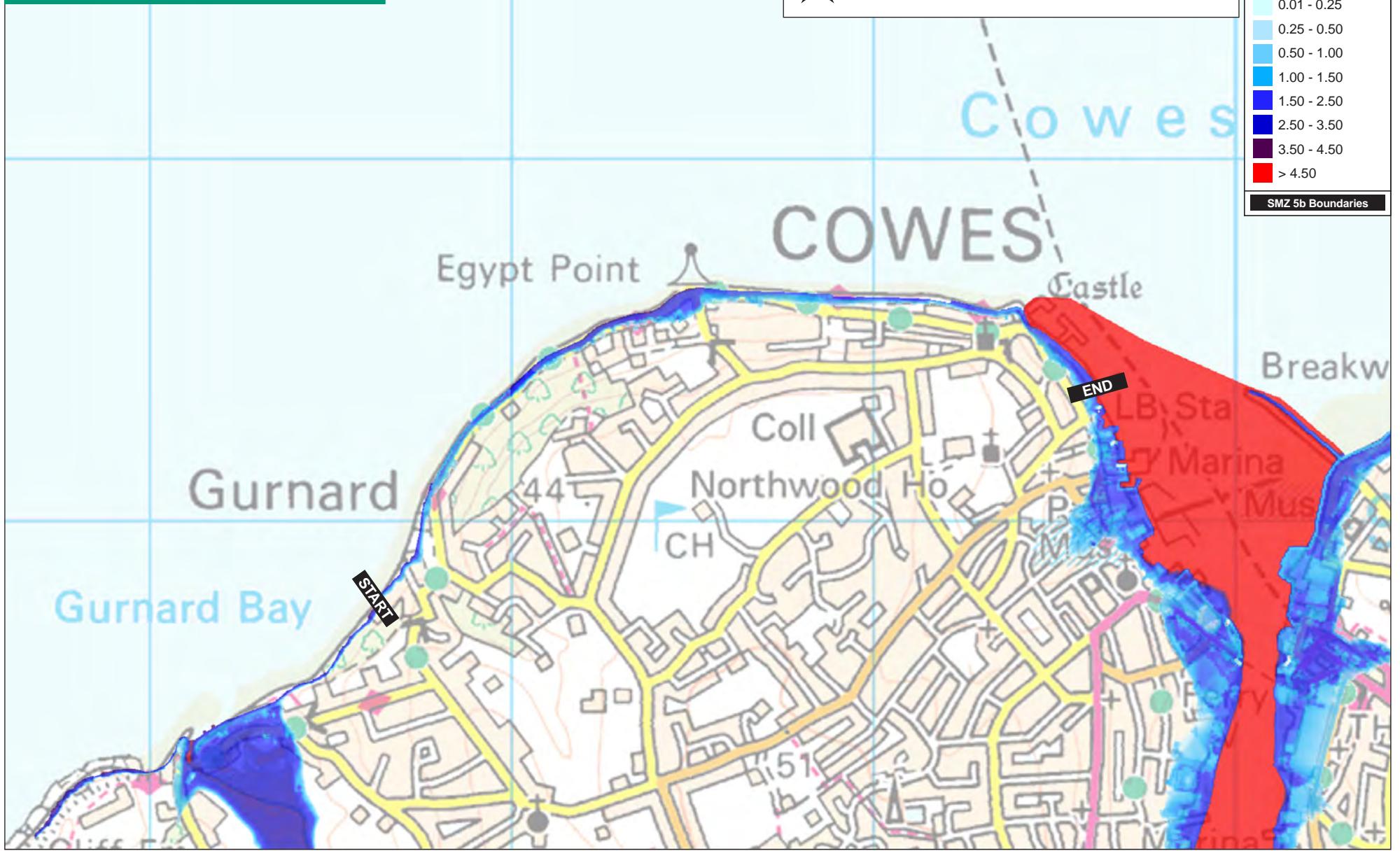
Maximum potential flood depths from a 1:200 year (0.5% annual chance) event with existing defences in place
